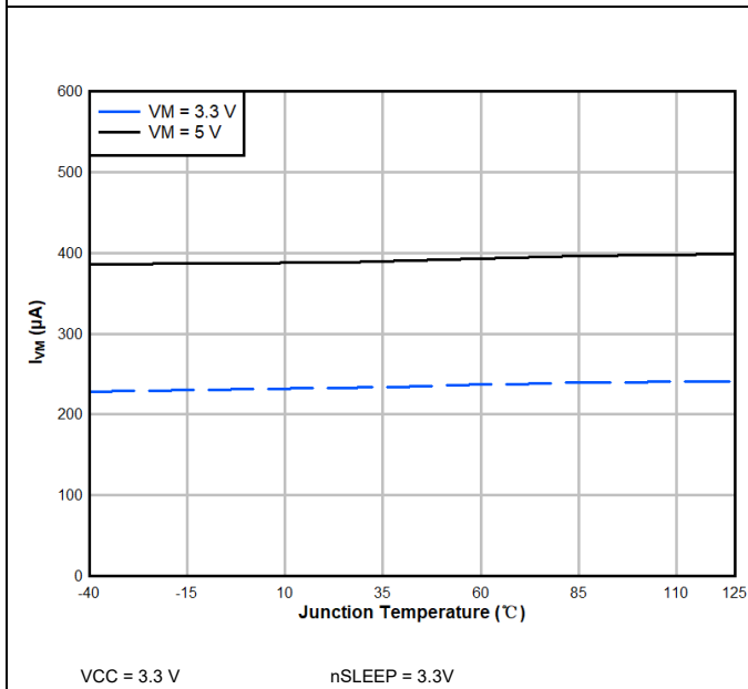
Figure 3. VM Operating Current vs Ambient Temperature
