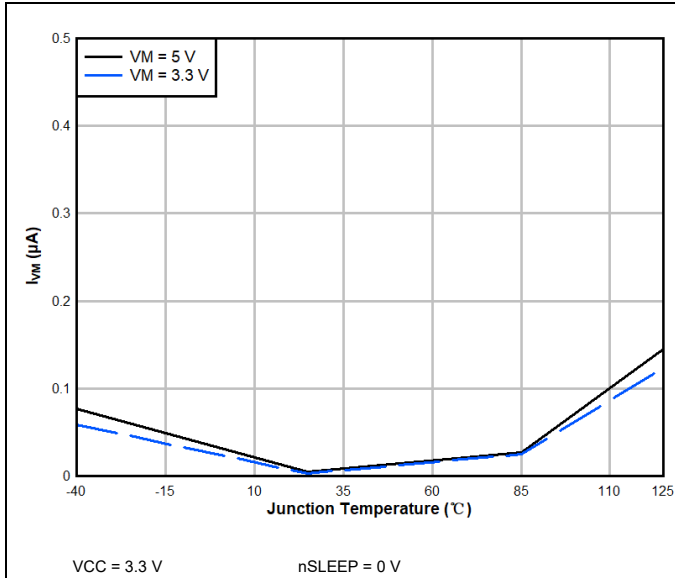
Figure 1. VM Quiescent Current vs Ambient Temperature
