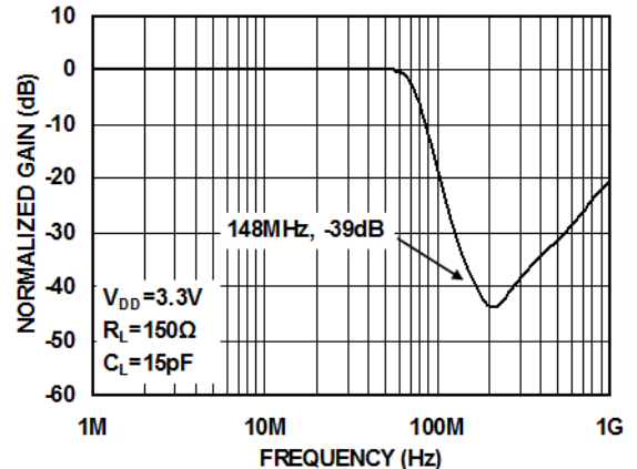
Figure8. Stop Band Attenuation
